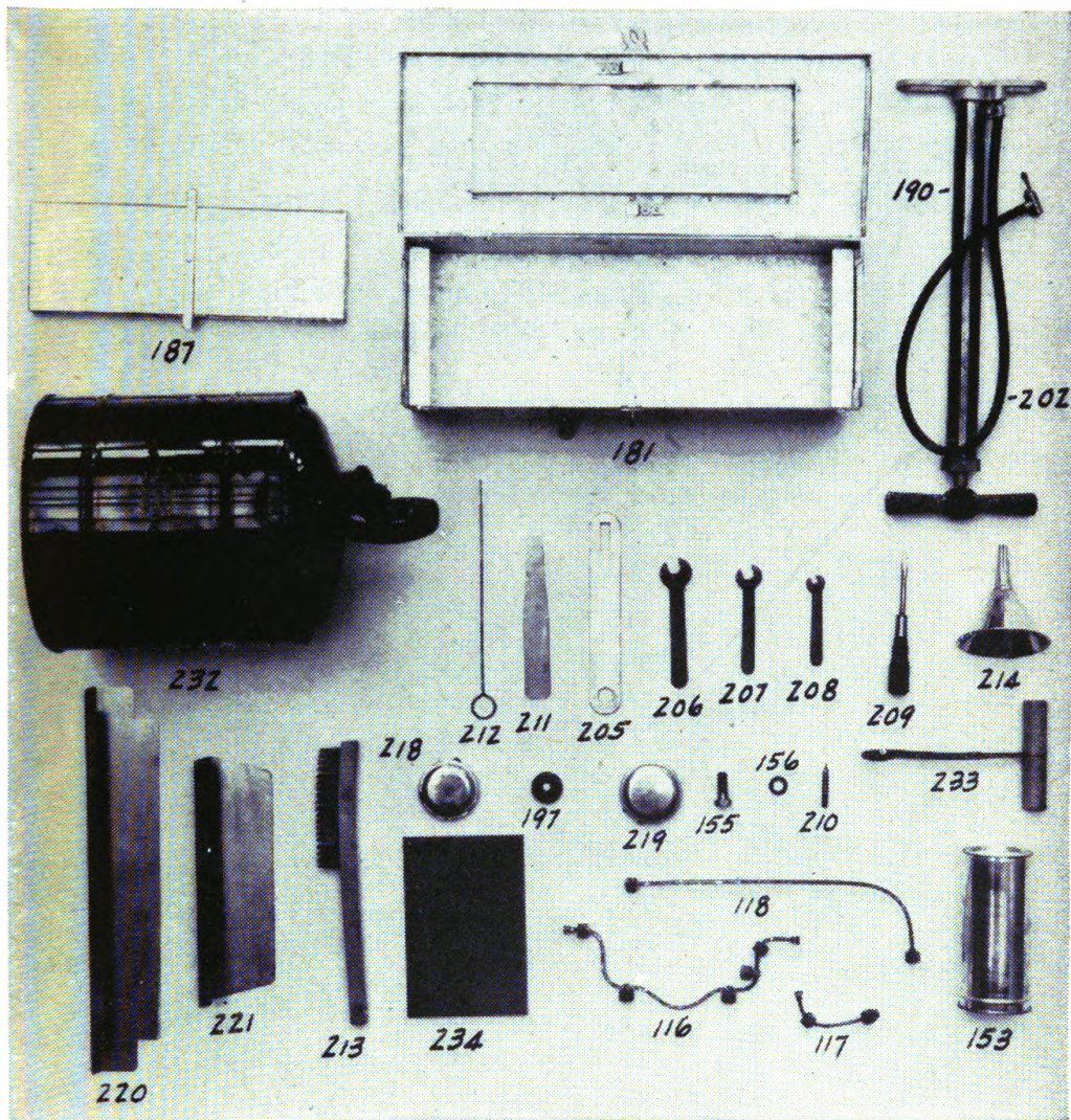
FIGURE 38.—Gasoline fire unit parts and tools—Continued.
